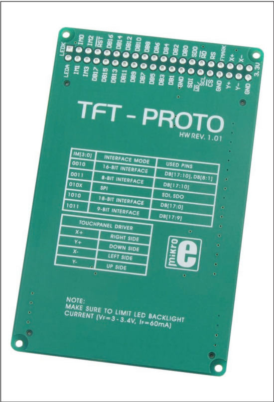
Figure 3: Back side of the TFT PROTO additional board
