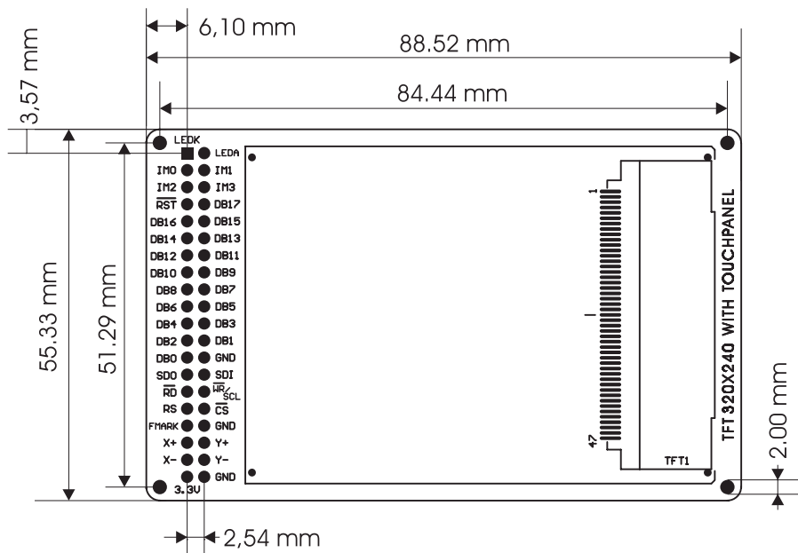
Figure 4: Dimensions of the TFT PROTO additional board
