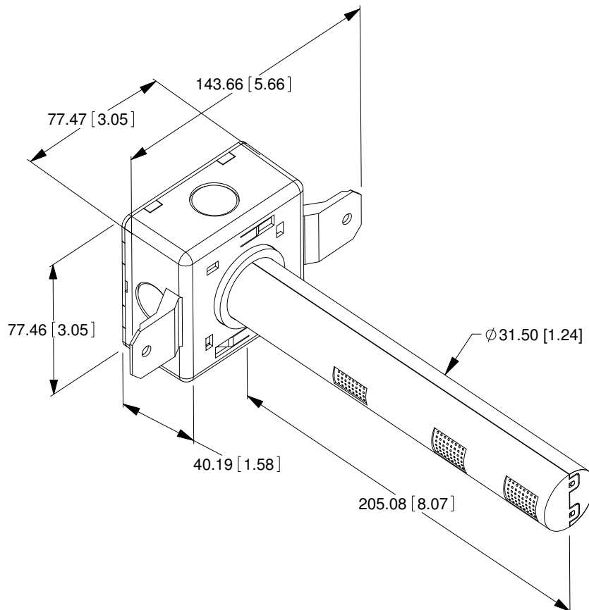
T8042 Dimensions (All Dimensions are in MM [Inch].)
