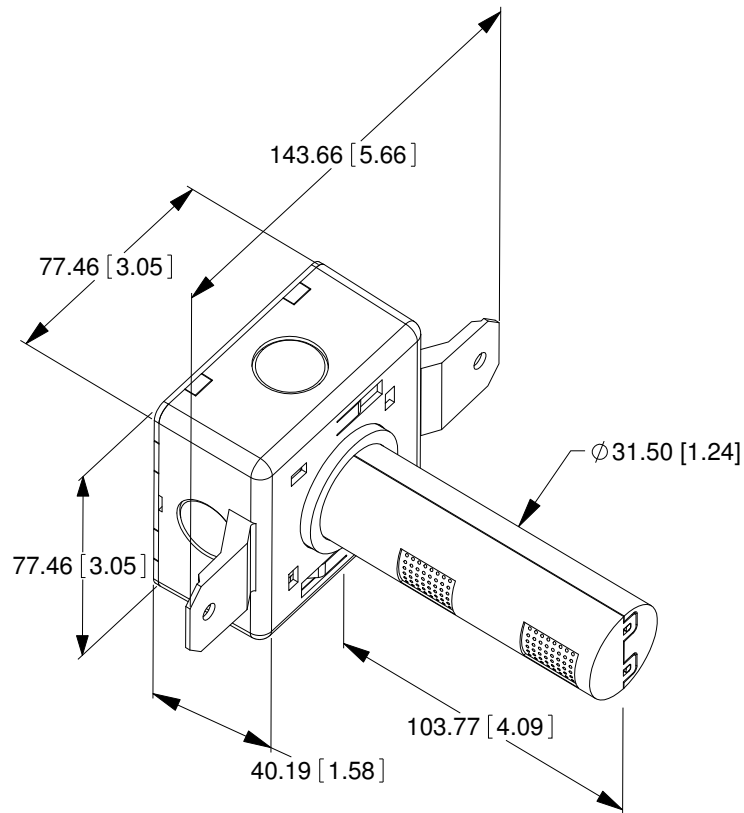
T8041 Dimensions (All Dimensions are in MM [Inch].)
