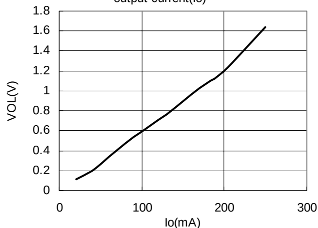
OUTpin low state voltage( V_{OL} ) vs. output current( I_O )
