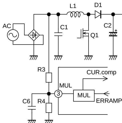
Fig.7 Multiplier circuit
