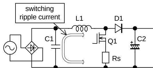
Fig.27 Input capacitor circuit
