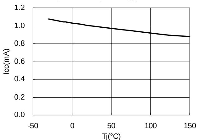
Operating power supply current( I_{CC} ) vs. junction temperature( T_J )
