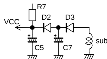
Fig.21 Vcc pin circuit (2)
