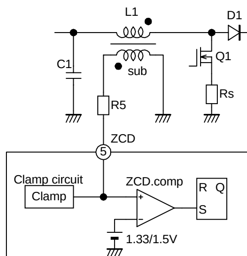
Fig.9 ZCD circuit
