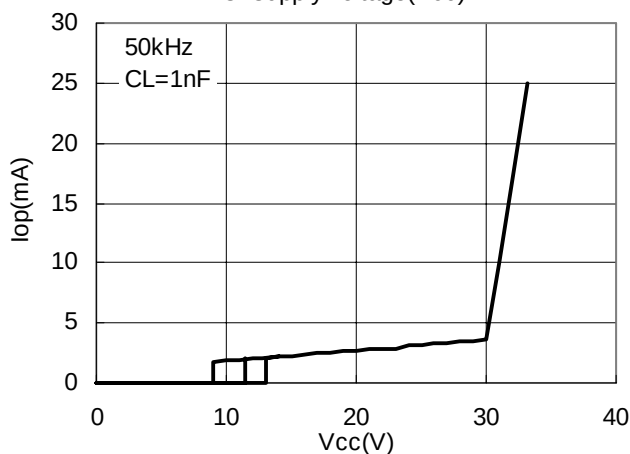
Dynamic operating power supply current( I_{OP} ) vs. supply voltage( V_{CC} )
