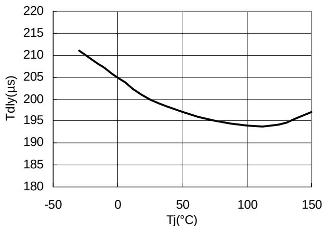
Restart timer deley time( T_{dly} ) vs. junction temperature( T_j )
