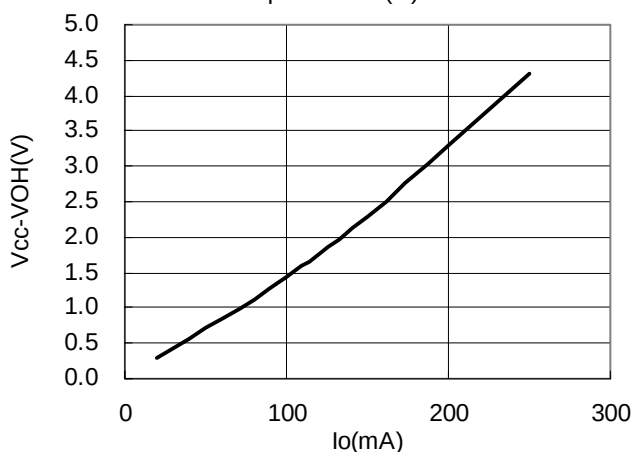
OUT pin high state voltage( V_{OH} ) vs. output current( I_O )
