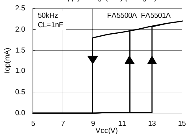
Dynamic operating power supply current( I_{OP} ) vs. supply voltage( V_{CC} ) (enlarged)
