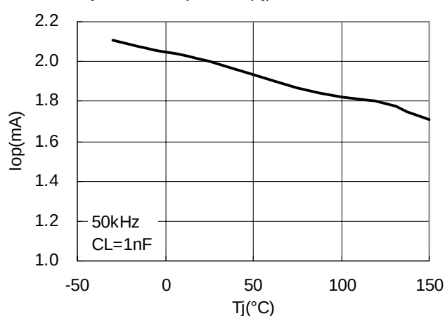
Dynamic operating power supply current( I_{OP} ) vs. junction temperature( T_J )
