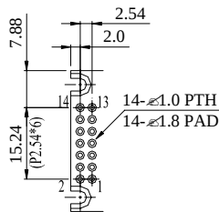
PIN DETAIL
