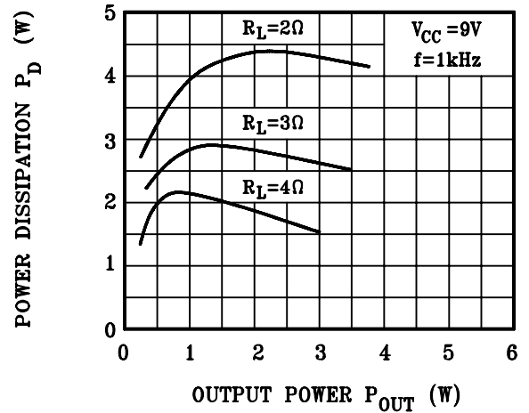
P_D - P_{OUT}
