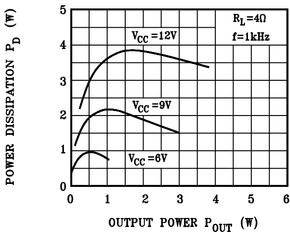
P_D - P_{OUT}
