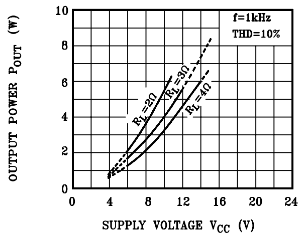
P_{OUT} - V_{CC}
