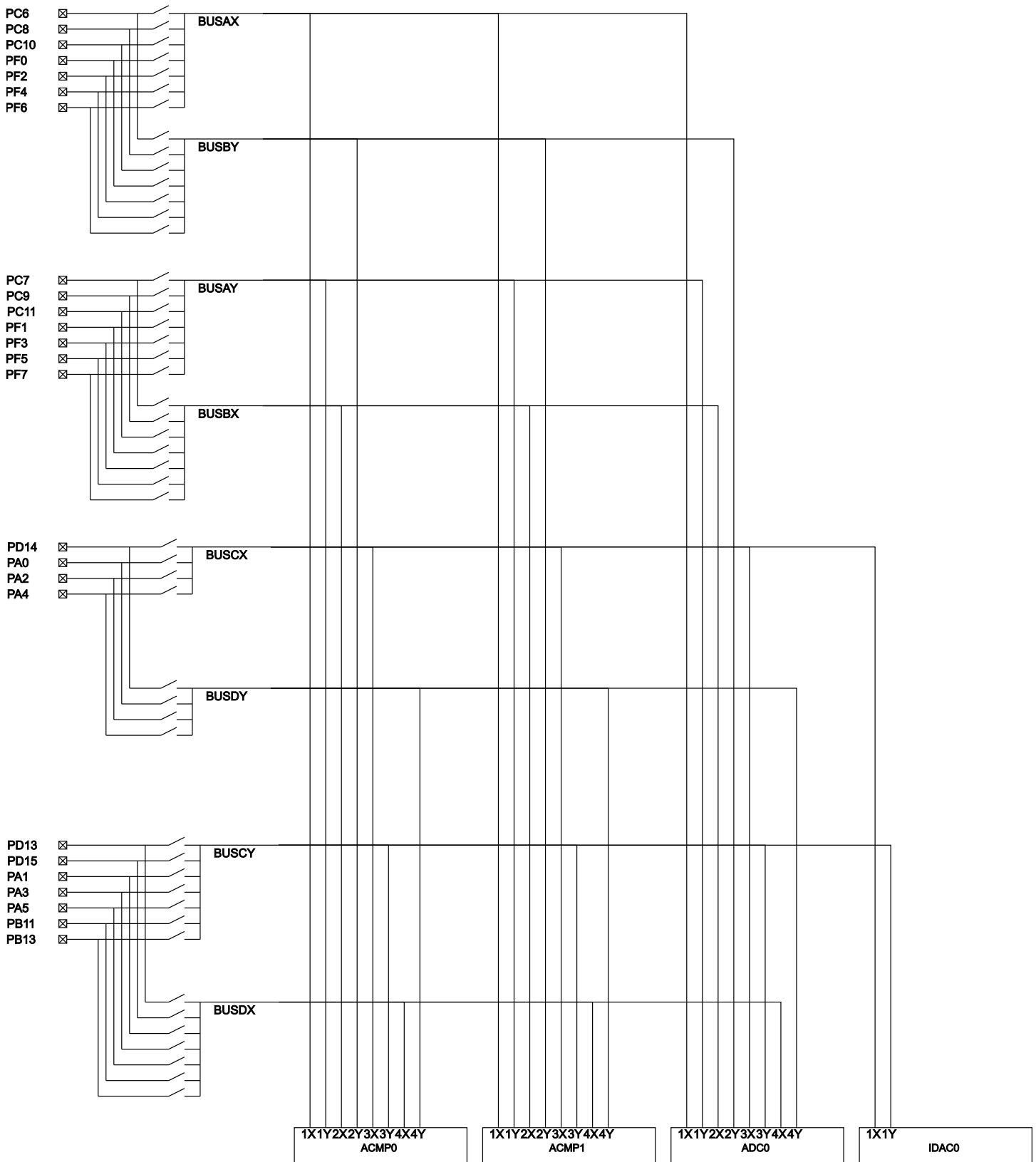
Figure 7.2. BGM111 APORT
