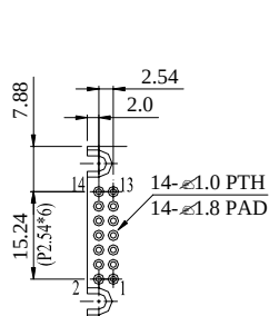
PIN DETAIL
