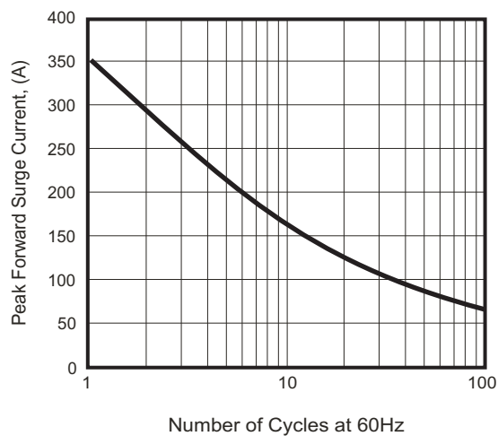
Fig.3 - Max. Forward Surge Current
